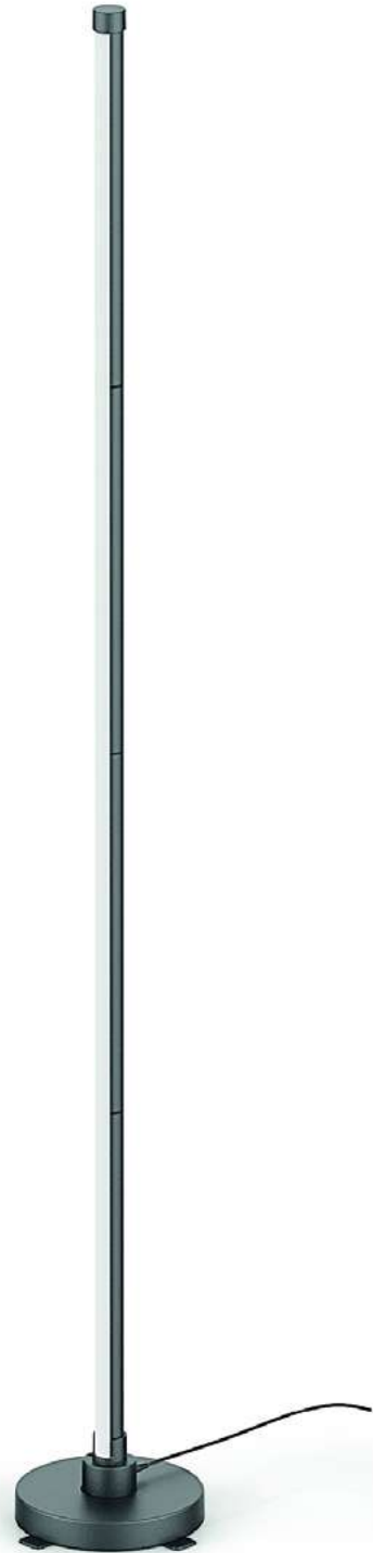
LED CORNER LIGHT DIGITAL RGB + W WITH MUSIC SENSOR 11.5W | 1 260lm | 120° | 1 475mm
