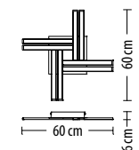
5317 PL-8 Q LED 48 W 3690 lm* 230 V
