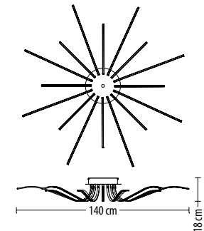
5330 PL-16 Q LED 82 W 6550 lm* 230 V
