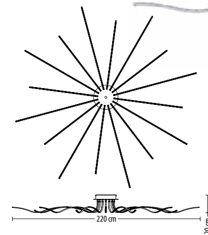
5254 PL-16 Q LED 140 W 10920 lm* 230 V
