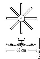
5585 PL-8 Q LED 35 W 2680 lm* 230 V
