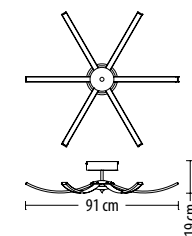
5586 PL-6 Q LED 43 W 3270 lm* 230 V
