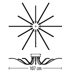
5256 PL-12 Q LED 52 W 4030 lm* 230 V
