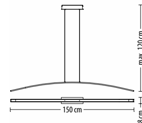
5304 Z-1 Q LED 25 W 1675 lm* 230 V
