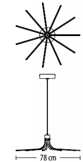
5840 Z-11 Q LED 57 W 4390 lm* 230 V
