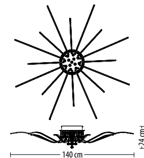
5331 PL-16 Q LED 82 W 6550 lm* 230 V
