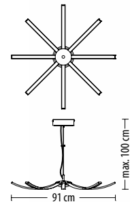
5580 Z-8 Q LED 57 W 4360 lm* 230 V
