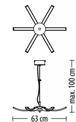
5583 Z-6 Q LED 26 W 2000 lm* 230 V
