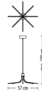
5841 Z-8 Q LED 32,8 W 2520 lm* 230 V
