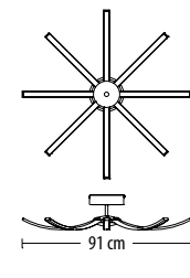
5584 PL-8 Q LED 57 W 4360 lm* 230 V
