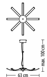
5581 Z-8 Q LED 35 W 2680 lm* 230 V
