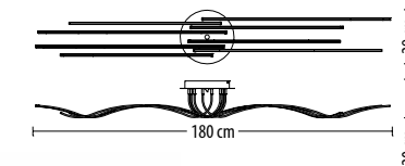
5253 PL-8 Q LED 70 W 5460 lm* 230 V
