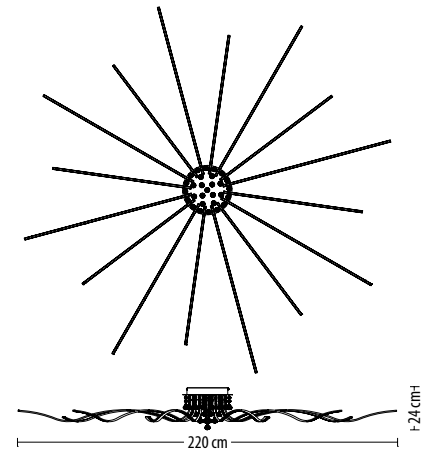
5255 PL-16 Q LED 140 W 10920 lm* 230 V
