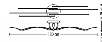
5251 PL-6 Q LED 47 W 3130 lm* 230 V
