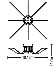
5259 PL-8 Q LED 35 W 2680 lm* 230 V
